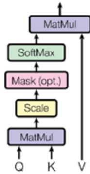
Figure 2. (left) Attention to scale product point. (right) multi-head attention consists of several layers of attention running in parallel (OpenAI, 2023).
