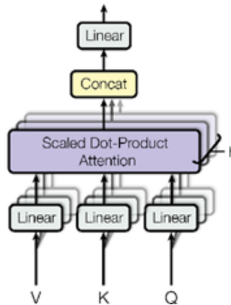
Figure 2. (left) Attention to scale product point. (right) multi-head attention consists of several layers of attention running in parallel (OpenAI, 2023).
