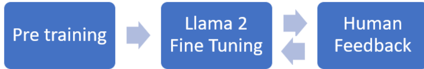
Figure 13. Training process.
